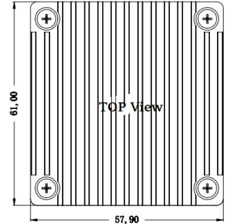
Standard+Heatsink 61*57.9*27.7mm
