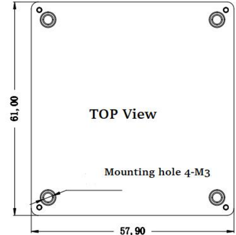
Standard 61*57.9*12.7mm
